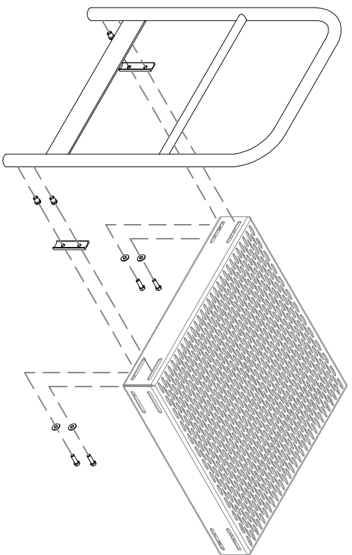
TYPICAL BOLTED CONNECTION
