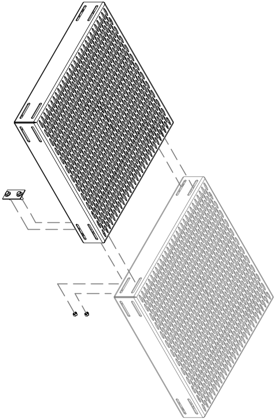
TYPICAL BOLTED CONNECTION
