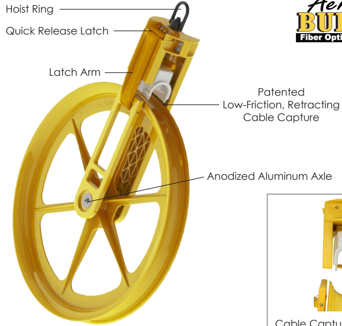
Cable Capture Retracts For Easy Loading and Unloading (Patent Pending)
